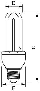
Economy Stick 23W CDL E27 220-240V
