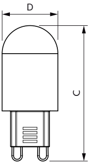
MV 110-240V 1.7W-25W 160lm 6500K G9 ND
