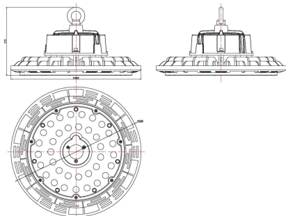
PA2-LED Indoor
