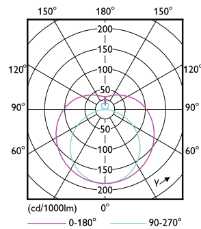
Light Distribution Diagram - MAS LEDtube 1200mm HO 26W 830 G5 VWV BR
