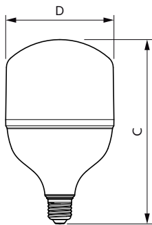
TForce 100-240V 40W 4800lm 6500K E27 ND
