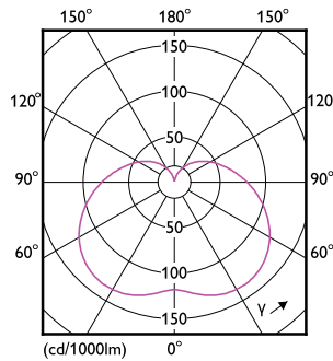
LEDTForce Core HB 40W Tshape E27 865 1
