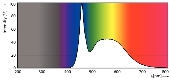
LEDTForce Core HB 30W Tshape E27 865 1
