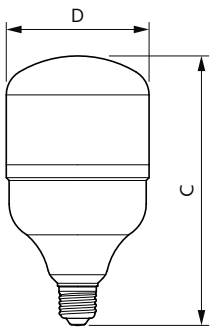
TForce 100-240V 30W 3800lm 6500K E27 ND
