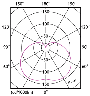
LEDTrueForce Core HB 30W Tshape E27 865 1
