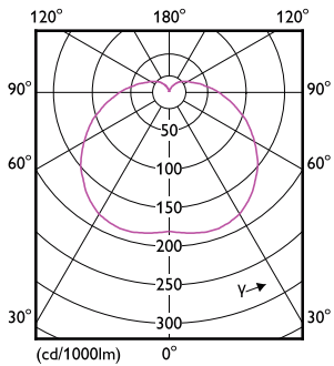
LEDTForce Core HB 24W Tshape E27 865
