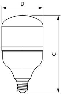
TForce 100-240V 24W 2800lm 6500K E27 ND
