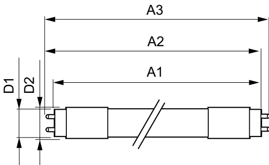
MasterConnect LEDtube IA 600mm HO 7W840 T8 BR
