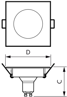
Kit S SSW GU10 5-50W 345lm 36D 2700K ND
