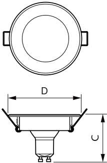
Kit R SSW GU10 5-50W 345lm 36D 2700K ND
