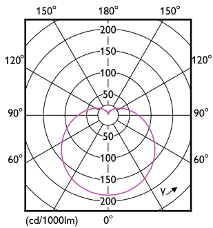
Light Distribution Diagram - LEDBulb 9W E27 4000K W 1PF/40 BR
