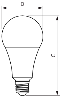
Bulb A80 15-32W 1800lm 6500K E27 ND N/A
