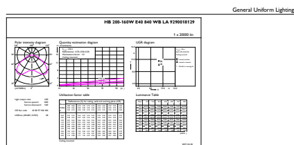
General Uniform Lighting CalcLux Photometrics 4.3 Philips Lighting B.V. Page 1/17
