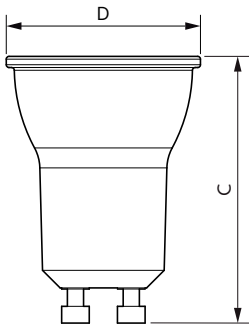
MR11 12V 3.3-25W 250lm 36D 2700K GU10 ND
