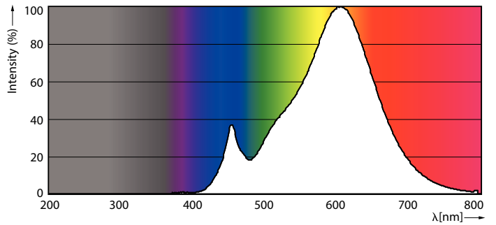
LEDspots 3,5W MR11 GU10 827 36D
