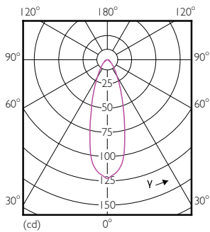
LEDspots 3,5W MR11 GU10 827 36D
